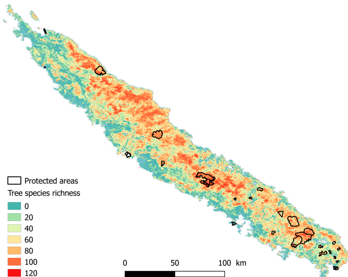
Figure 5. Species richness of trees with \text{dbh} \geq 10 cm predicted from a single carefully selected scene (days 245 to 252 of 2004) and the protected area network in New Caledonia.
